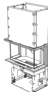
Building frame B
