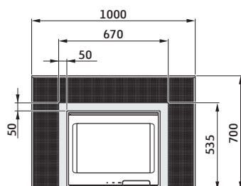
Frame and decor grille
