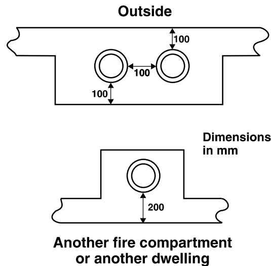
Diagram 20 Wall thicknesses for masonry and flueblock chimneys
