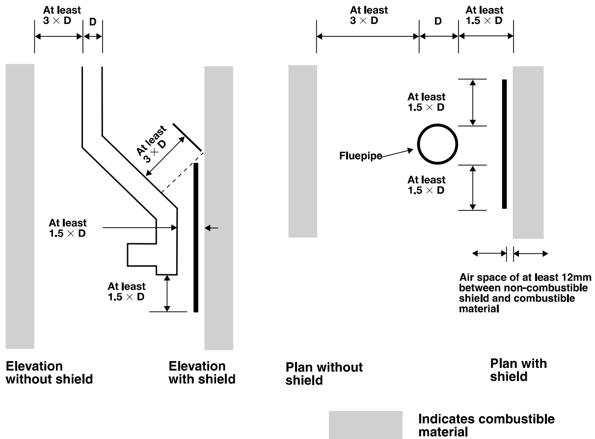
Diagram 19 Protecting combustible material from uninsulated fluepipes for solid fuel appliances
