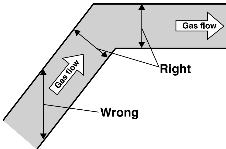
Diagram 7 Measurement of flues and ducts
