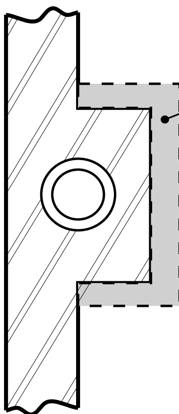
Diagram 12 Material change of use: fire protection of chimneys passing through other dwellings
