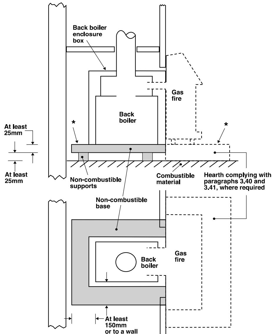
Diagram 36 Bases for back boilers (installation using a proprietary back boiler enclosure shown)
