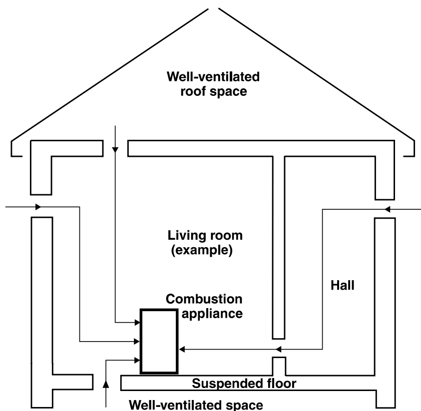
Diagram 10 Location of permanent air vent openings, some examples
