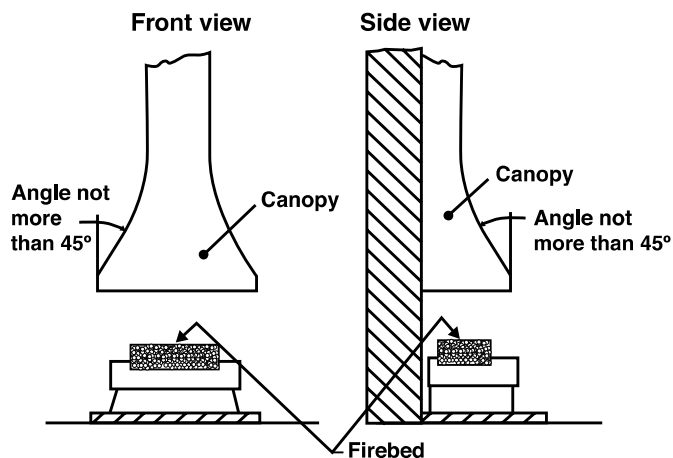
Diagram 23 Canopy for an open solid fuel fire
