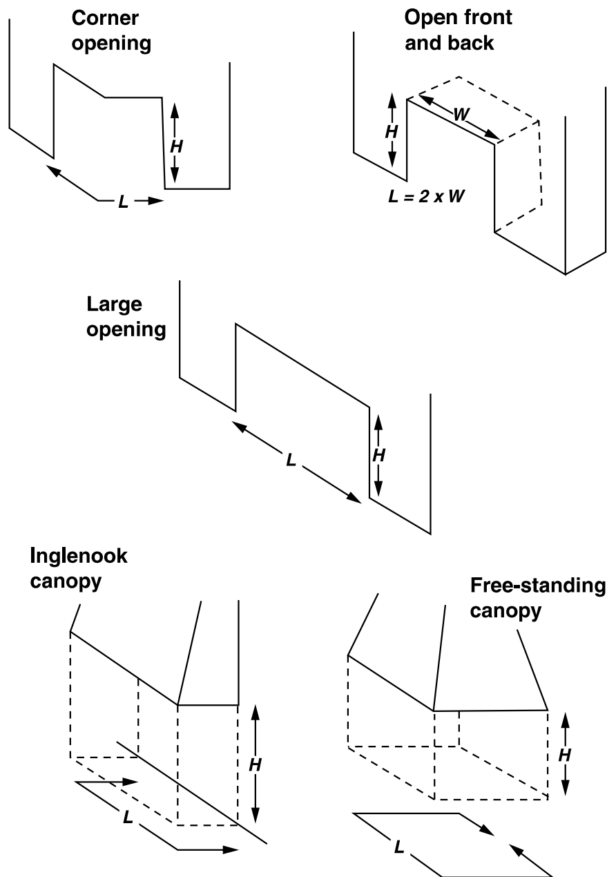
Diagram 45 Large or unusual fireplace openings. (Note: for use with this Appendix, measure L, H and W in mm)
